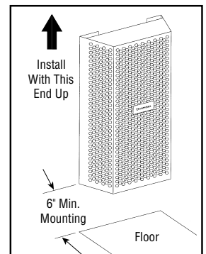
Figure 1 — Mounting
