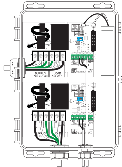
FIGURE 1. The GPT 130 wiring layout
