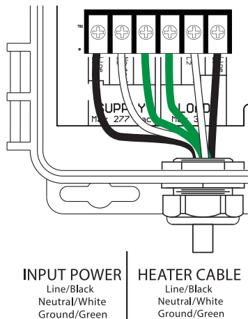
FIGURE 3.2 Contractor Connections
