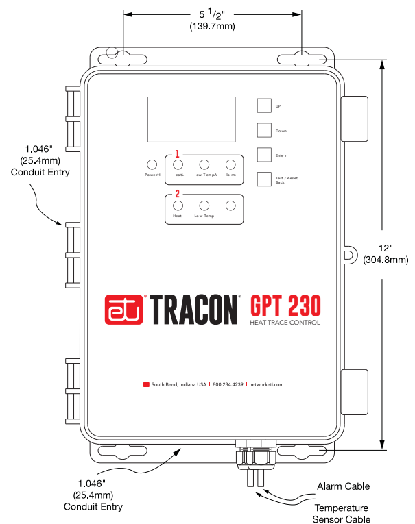
FIGURE 2. Mounting Dimensions
