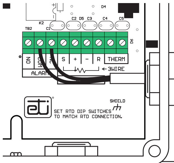
Wiring to Normally Closed Alarm Contact
